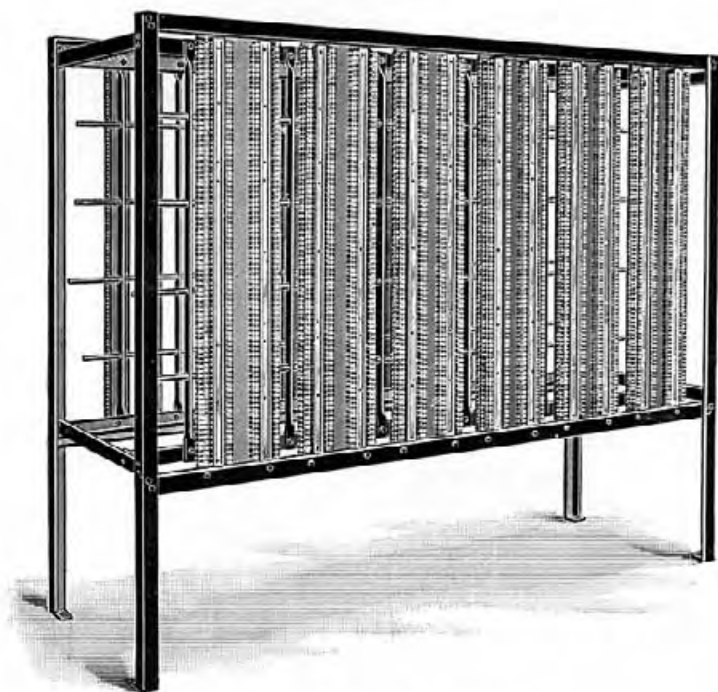
Showing Lightning Arrester. Size, 74\frac{1}{8} in. long, 24 in. wide, 60 in. high.
