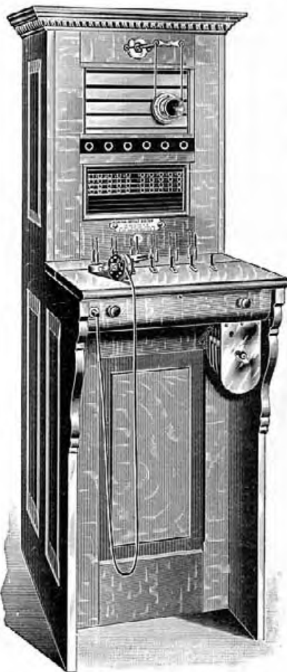
No. 102. 50-line “Central Energy” Switchboard.
