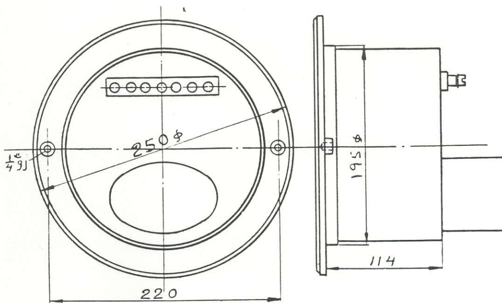
Wattmeter, type II W 250.
